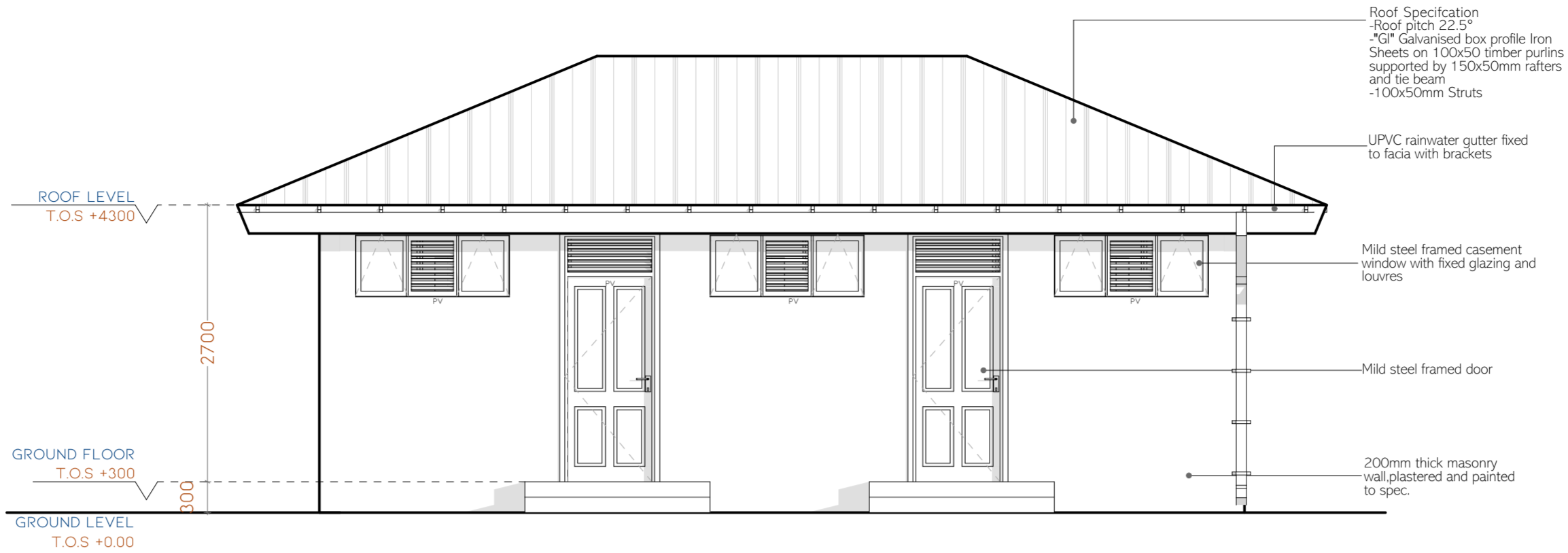
ELEVATION 01 SCALE 1:50
