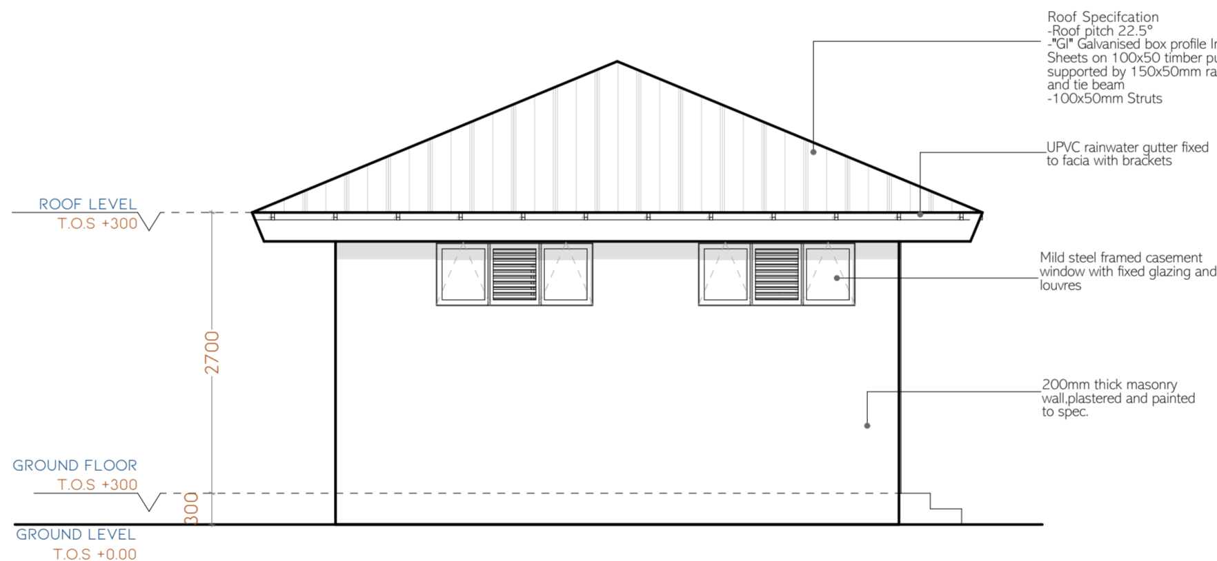
ELEVATION 02 SCALE 1:50
