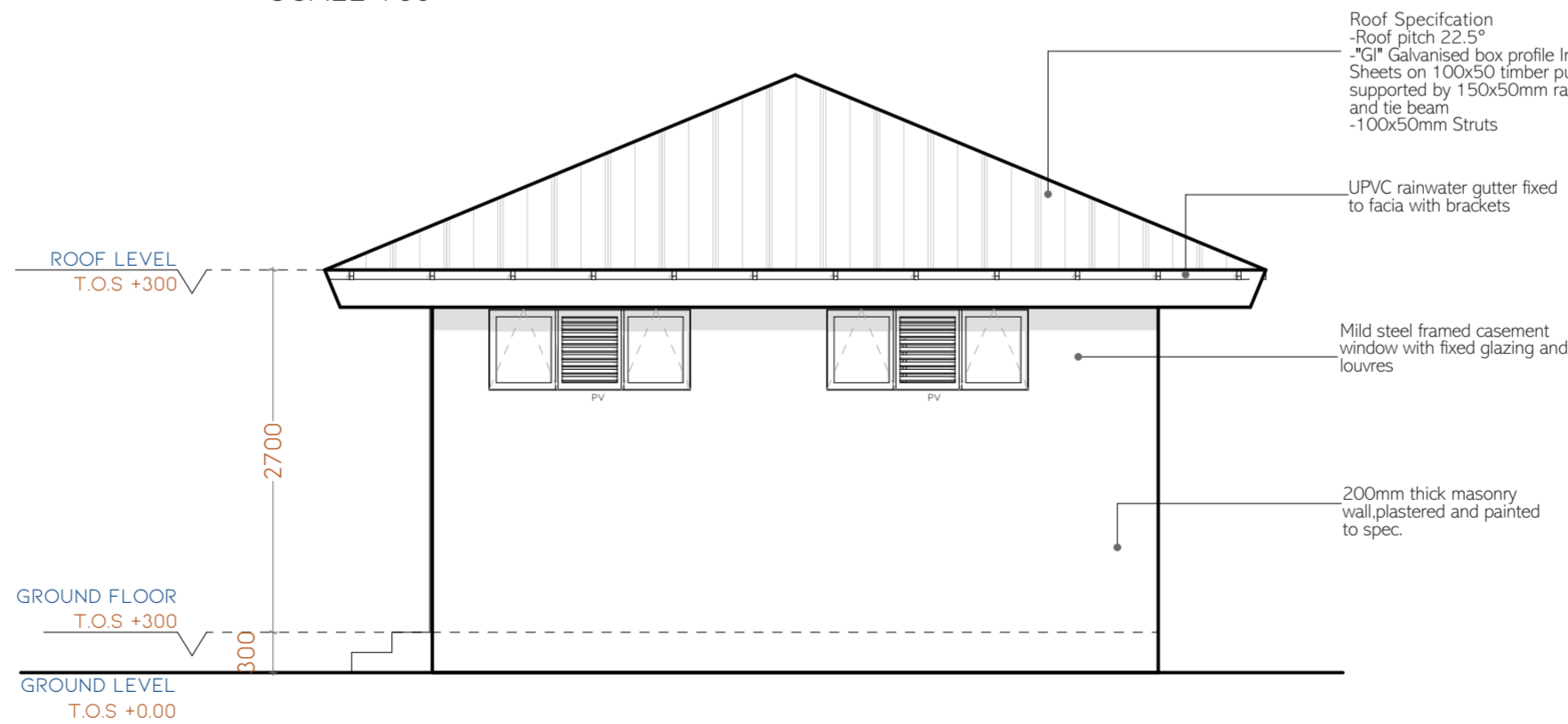
ELEVATION 04 SCALE 1:50
