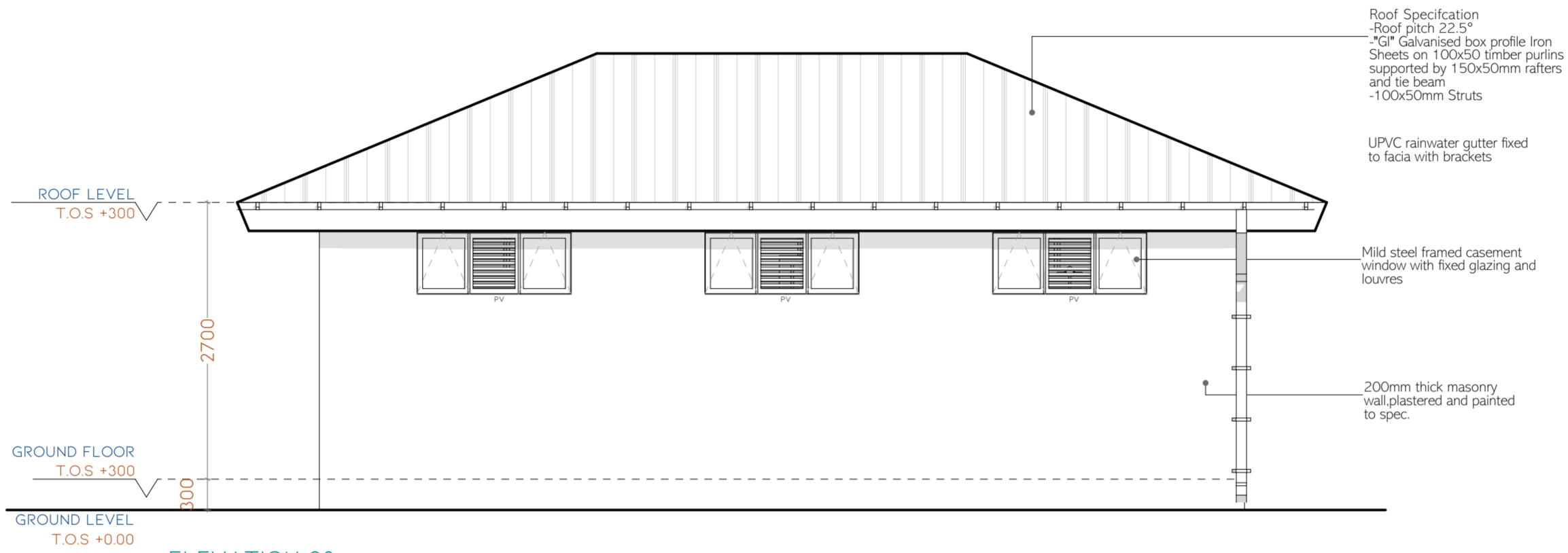
ELEVATION 03 SCALE 1:50
