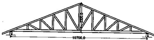
TRUSS 2
