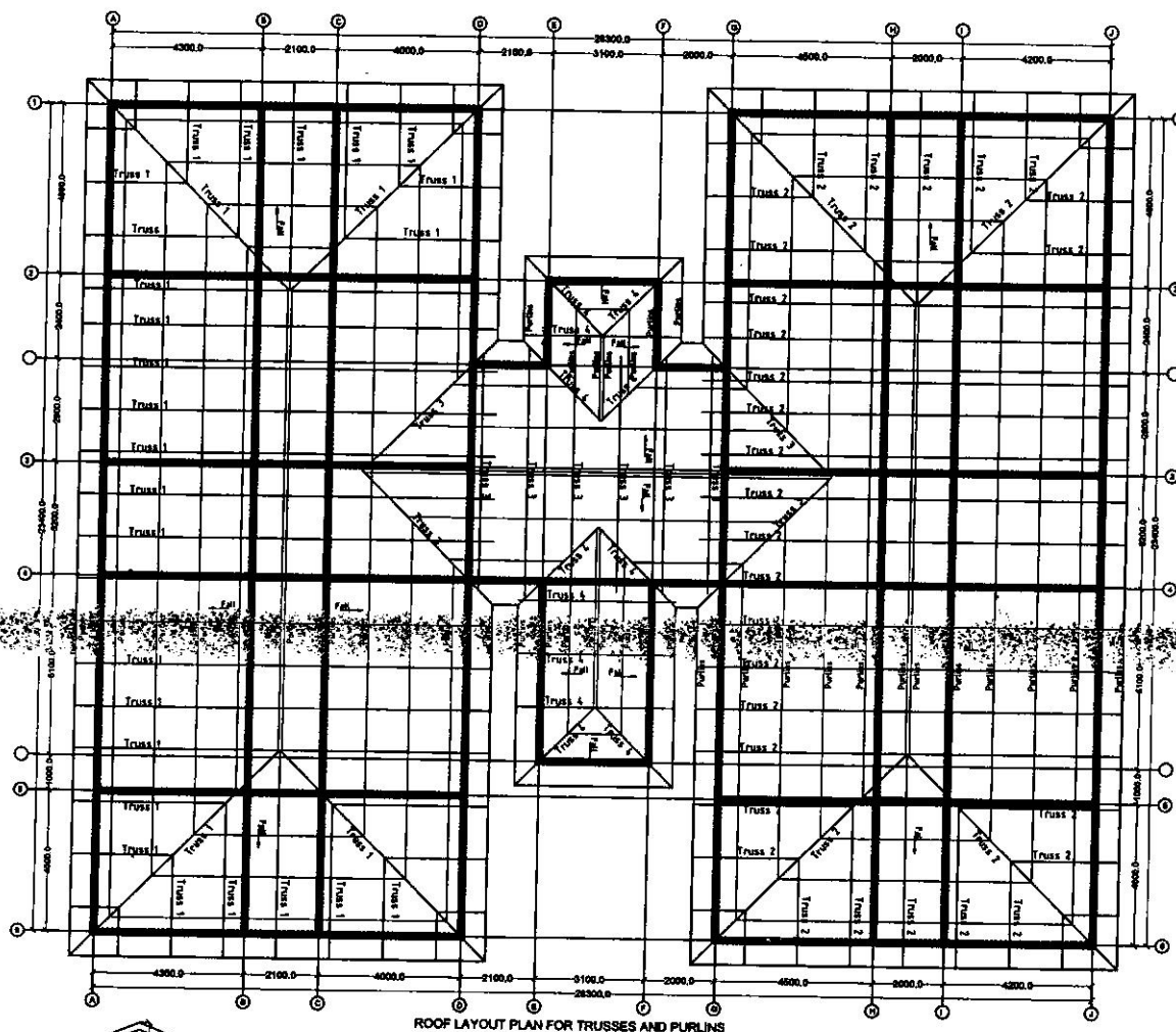
ROOF LAYOUT PLAN FOR TRUSSES AND PURLINS
