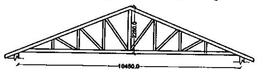
TRUSS 1
